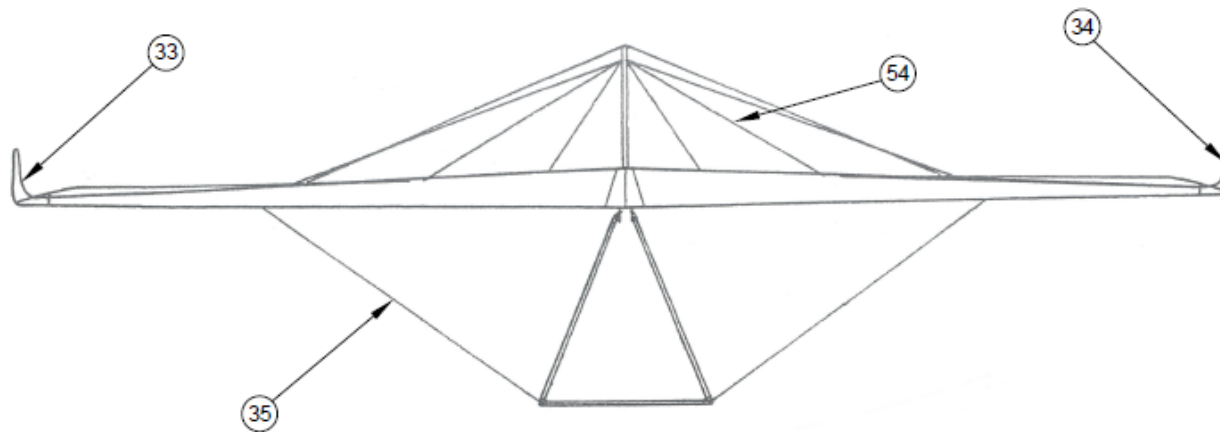
FRONT ELEVATION
