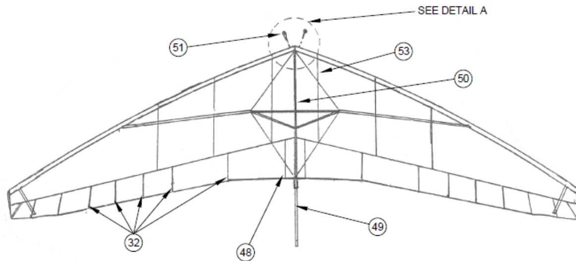
UNDERSIDE ELEVATION
